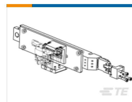
TE Part # 1-2326143-0 RETROFIT KIT, INFINITE SPLICE
