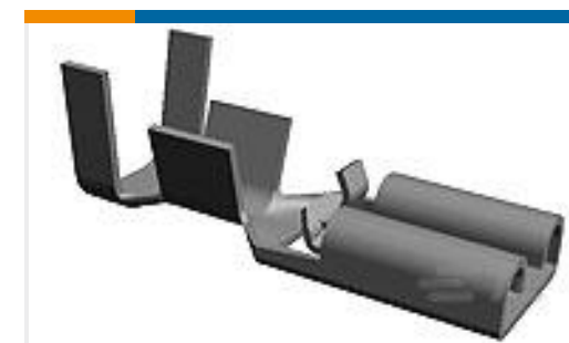
TE Part #1217113-1 PL 187 TERMINAL RECEPTACLE 22-18 AWG BR
