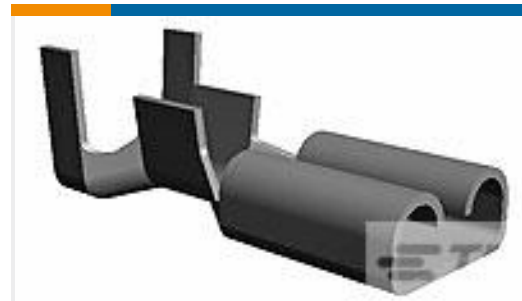
TE Part #62138-1 187 FASTON REC 24-20 TPBR
