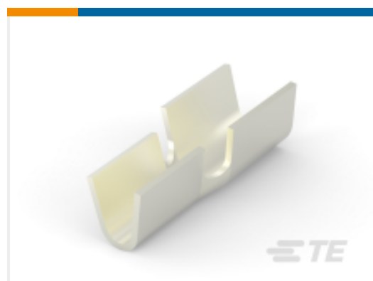
TE Part # 61021-1 SPLICE 18-16 AWG .0126 NPST
