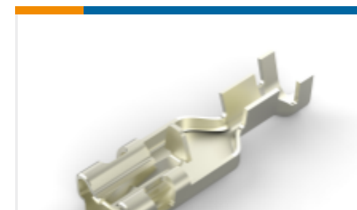
TE Part #170021-3 SHUR PLUG REC 20-16AWG BRIGHT DIP OIL BR
