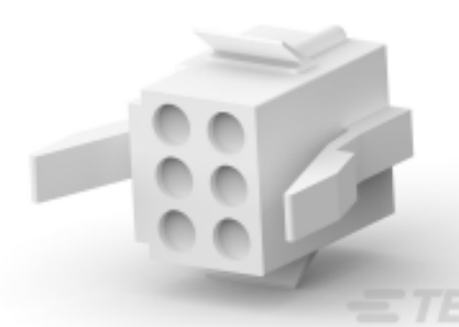
TE Part # 1-171196-0 6 POS MATE-N-LOK S
