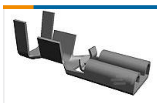
TE Part #1217113-1 PL 187 TERMINAL RECEPTACLE 22-18 AWG BR
