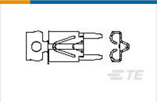
TE Part #63994-1 FASTON 205/250 PCB MOUNTED TPBR
