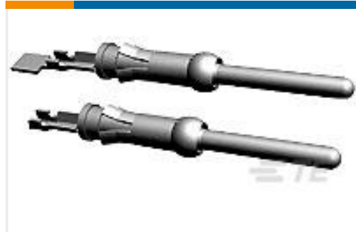
TE Part #66099-1 III+ PIN,18-16,30AU>10,LP
