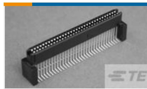
TE Part #120524-1 1FHR,64,30A/P,S,N,S14,15
