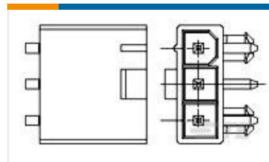
TE Part #2029150-5 5P R/A HDR VAL-U-LOK V2 W/P
