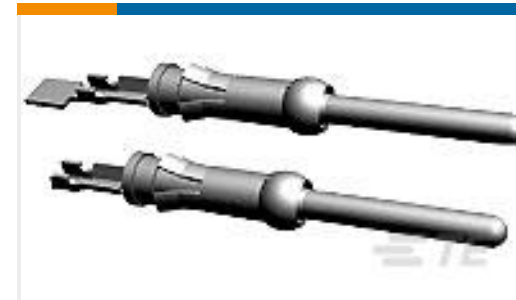
TE Part #66103-2 III+ PIN,24-20,TIN-LEAD,LP
