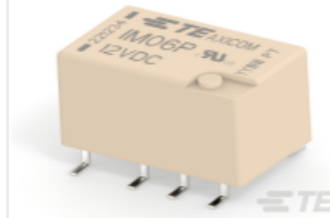
TE Part #5-1462039-6 IM06PGR=IM RELAY 140mW 12V
