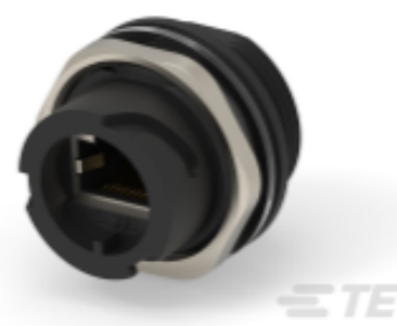
TE Part #2355443-2 RJ45 CAT5e PANEL MOUNT SOCKET (PBT)
