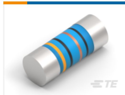
TE Part #3-2176314-0 MELF SMA_A 27K 0.1% 15PPM 0102 0.3W
