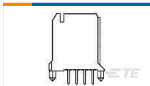
TE Part # 5223655-2 2MM FB,4RV,REC,ASY,048,SL,4.25
