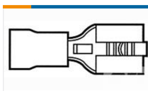
TE Part #640905-2 RECEPT,PIDG FASTON 16-14 250
