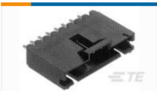
TE Part #6-103669-1 12 MTE HDR SRST LATCH W/HLDWN
