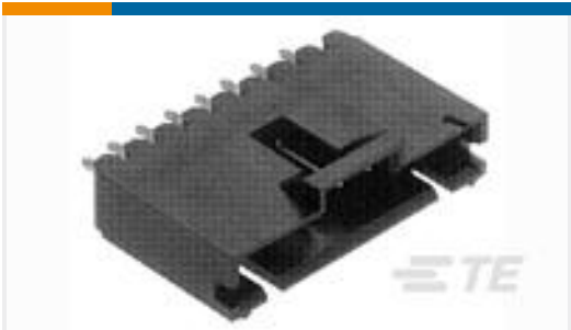
TE Part #103735-3 04 MTE HDR SRST LATCH .100CL
