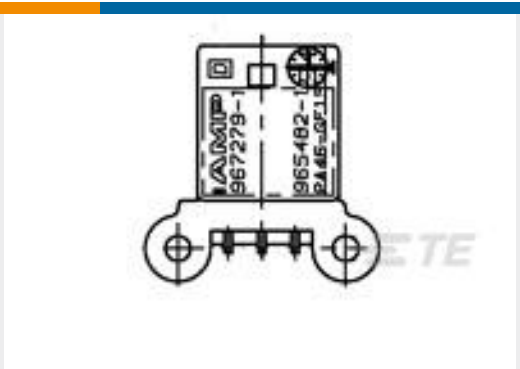
TE Part #967279-4 3pos MQS .63 header 90deg THR
