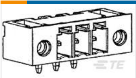
TE Part #284539-8 8 POS TERMI-BLOK 900 W.S.F. 3,
