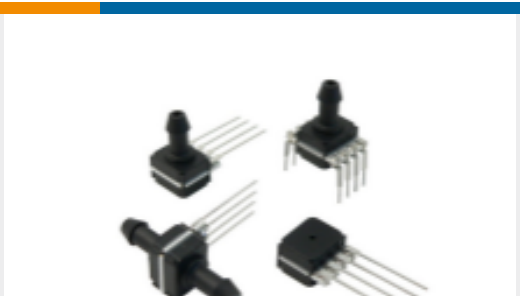
TE Part #2003626-F HMIB2X5UZ7H3; PRES; 0...2,5bar; 3V; DIL
