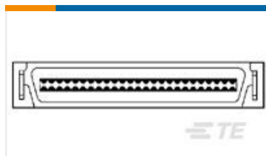
TE Part #1-1734101-7 Champ050 series, 50 pos,30u" Au, 3.30 H
