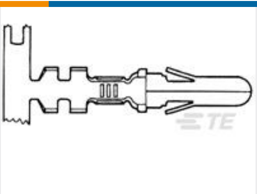
TE Part #350391-1 .140 DIA PIN 14-10 PTPBR L/P
