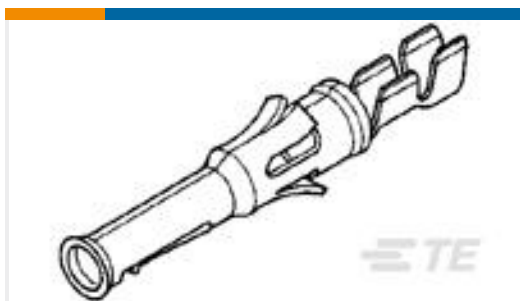
TE Part #66580-2 TYPE VI SKT CONT, MULTI-MATE
