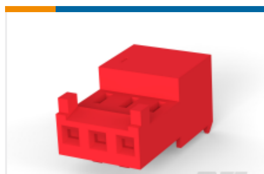
TE Part #3-643816-5 Nylon Tin Plated Receptacle: 2.54 mm, with Mating Alignment, MTA 100
