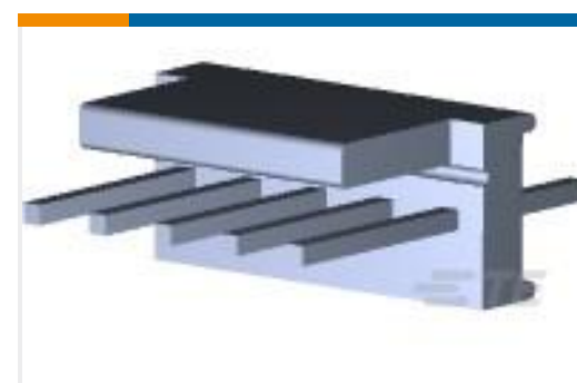
TE Part #640454-5 05P MTA100 HDR ASSY SQ STR POL
