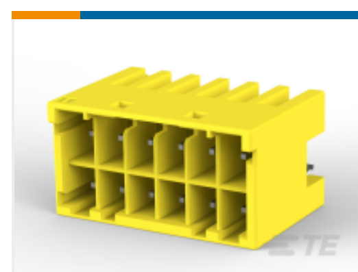
TE Part # 4-1971906-6 HEADER ASSY 12POS,KEYING-D, NEW GIC3.3
