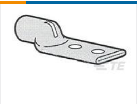
TE Part #326800 TERMINAL,AMPOWER 1/0 3/8
