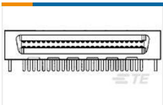
TE Part #5-5175474-7 .050CL,CHAMP,R/TANG RCPT,60POS
