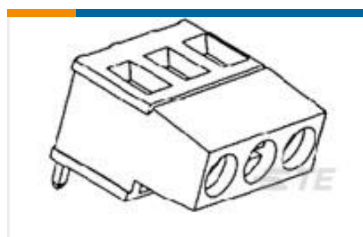
TE Part #282851-2 TERMI-BLOK PCB MOUNT 180 2P.5
