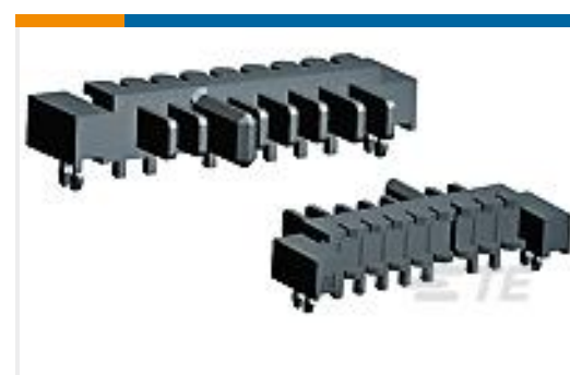
TE Part #1827654-2 2mm pitch Battery Plug Assy. 7P. H=4.0
