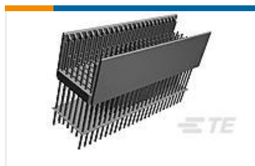
TE Part #188835-1 Z-PACK/B M-HDR 154P.
