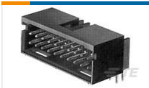
TE Part #6-103166-0 24 MODII HDR DRRR SHRD LF
