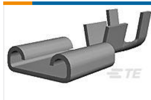
TE Part #170095-1 250 FASTON,REC.,22-18 AWG,TPPB
