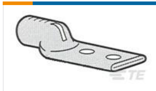
TE Part #327290 TERMINAL,AMPPOWER 600MCM 1/2
