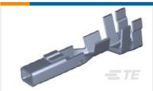
TE Part #179592-1 AMP POWER D/LOCK REC CONT. LP
