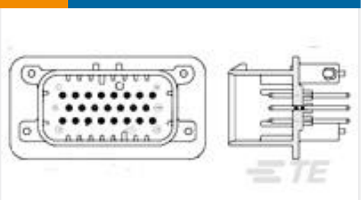
TE Part #1-776231-1 35POS,PIN DIA 1.3,HDR ASSY, 180DEG,COD 1
