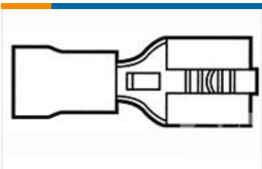
TE Part #8-640905-1 RECEPT,PIDG FASTON 16-14 250
