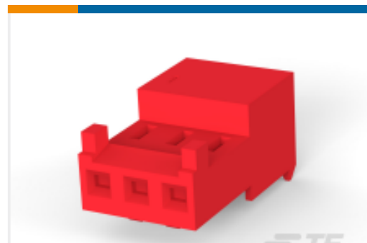
TE Part #3-643814-4 Nylon Tin Plated Receptacle: 2.54 mm, with Mating Alignment, MTA 100
