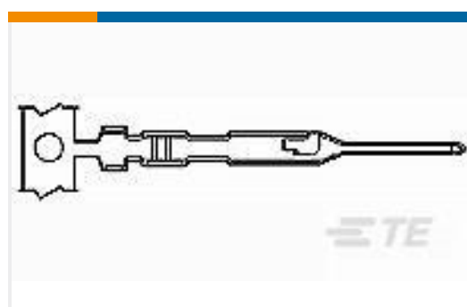
TE Part #104505-3 MTE PIN LP
