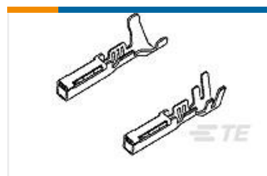
TE Part #175180-1 040 MULTILOCK REC CONT PRE-TIN
