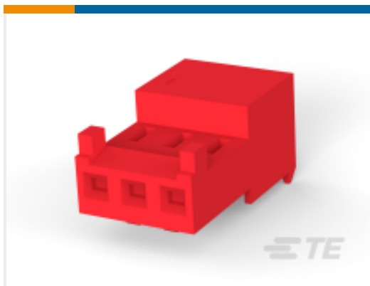
TE Part #4-643815-2 Nylon Tin Plated Receptacle: 2.54 mm, with Mating Alignment, MTA 100
