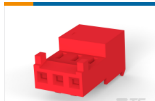
TE Part #3-643813-3 Nylon Tin Plated Receptacle: 2.54 mm, with Mating Alignment, MTA 100
