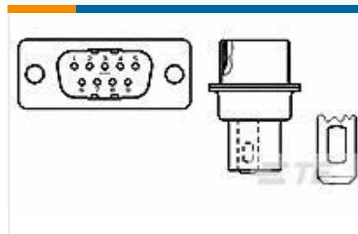
TE Part #215711-1 09P.HDP20 PLUG ASSY
