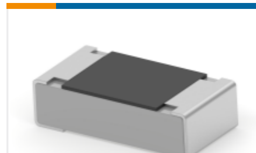
TE Part #2-2176340-5 CRGCQ 0603 10K 5%
