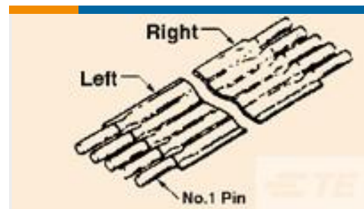
TE Part #3-640426-7 07P MTA156 CONN ASSY 18AWG ORA
