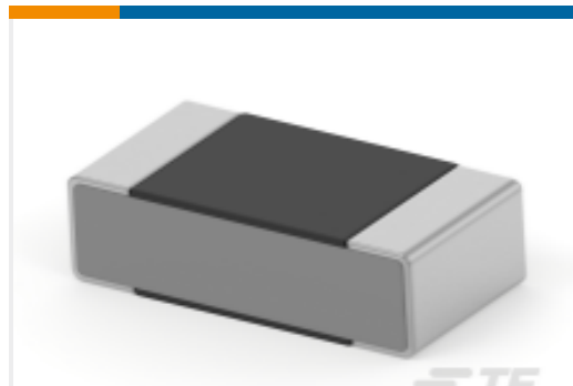
TE Part #6-2176326-1 CRGP 0603 1M0 1%
