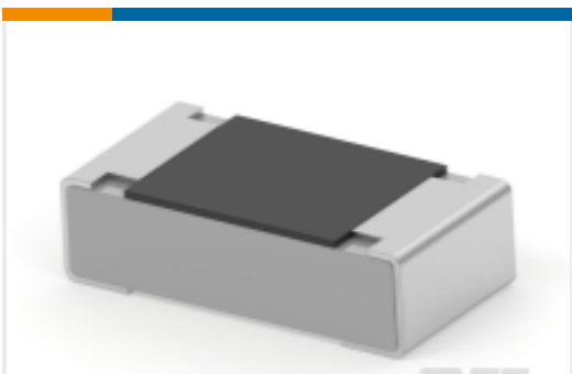
TE Part #2176340-9 CRGCQ 0603 22R 5%
