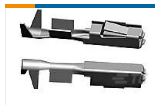
TE Part #5-928999-1 MQS0,63 Sn rec LL unseal. >0,2-0,35
