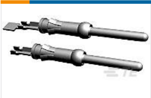
TE Part #66400-1 III+ PIN,24-20,TIN-LEAD,LP
