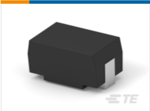
TE Part #1879011-1 SMD Power Resistor: 7 Watt, 200-2M Ohm
