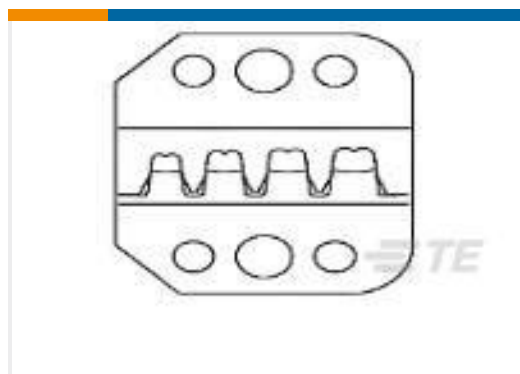
TE Part #58541-2 PRO-CRIMPER HAND TOOL DIE
