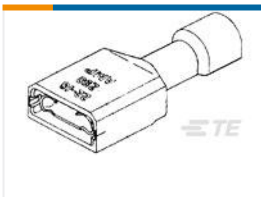
TE Part #3-350820-2 ULTRAFast 250 ASSY REC 16-14 TPBR LP
